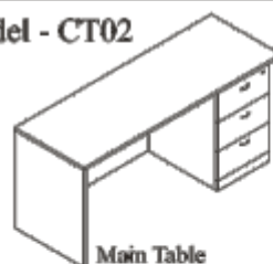
Main Table Size : 1800Lx750Dx750H
